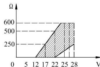
Load diagram
